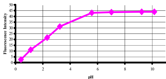
Fig. 1. Influence of pH on eosin fluorescence intensity
