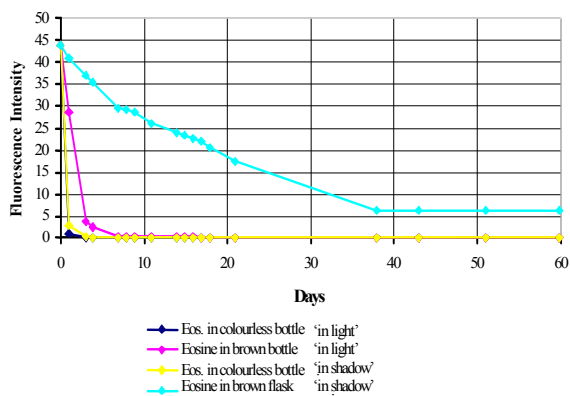
Fig. 3. Decay of the fluorescence of eosin in aqueous solutions exposed to different conditions of daylight
