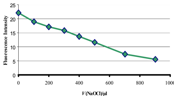
Fig. 2. Decay of eosin fluorescence in water solutions containing sodium hypochlorite
